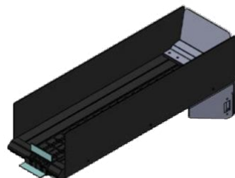
interner Lift 510 x 150 mm
